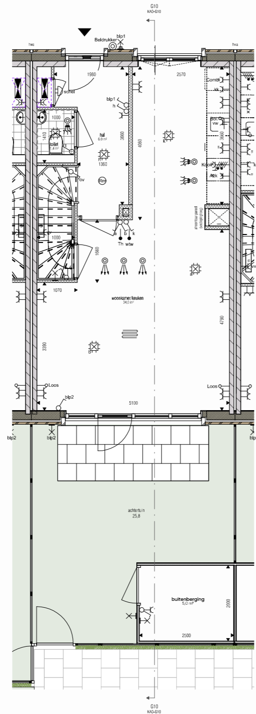
BNR G10_00 begane grond 1:100
