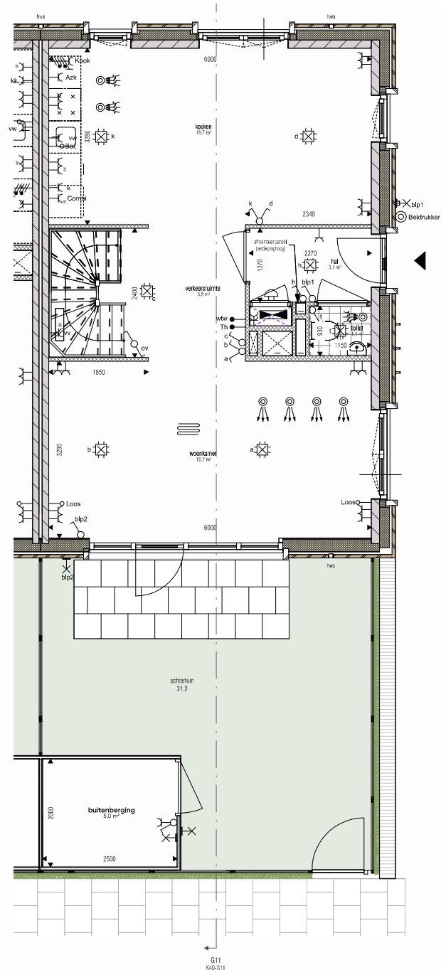
BNR G11_00 begane grond 1:100
